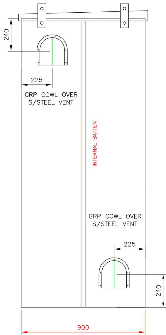
LEFT HAND ELEVATION
