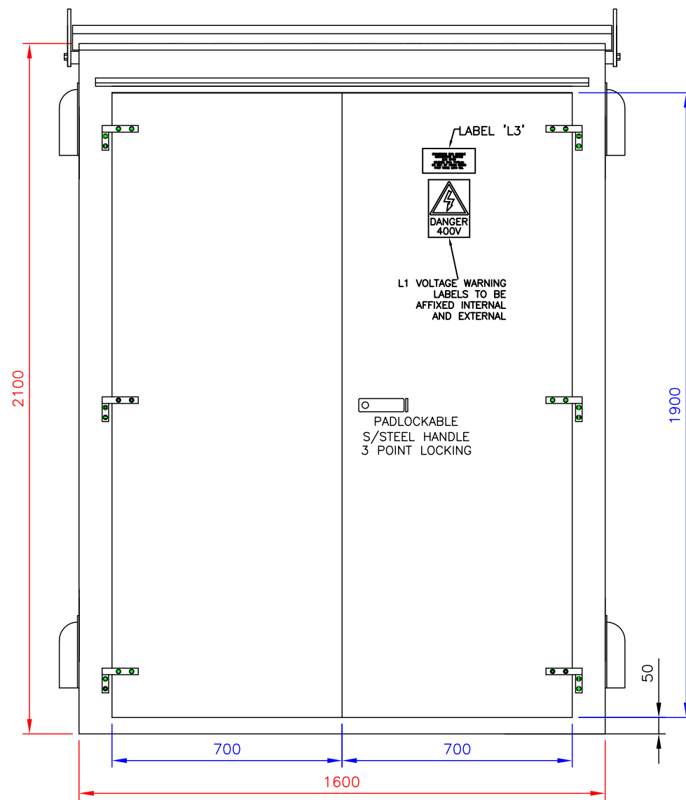
FRONT ELEVATION
