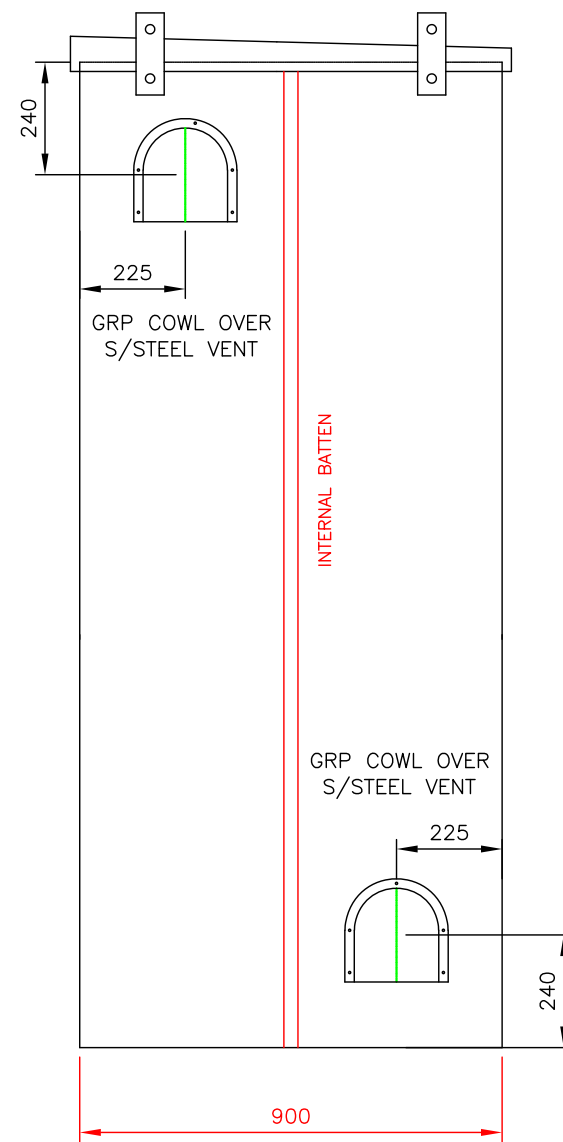
RIGHT HAND ELEVATION
