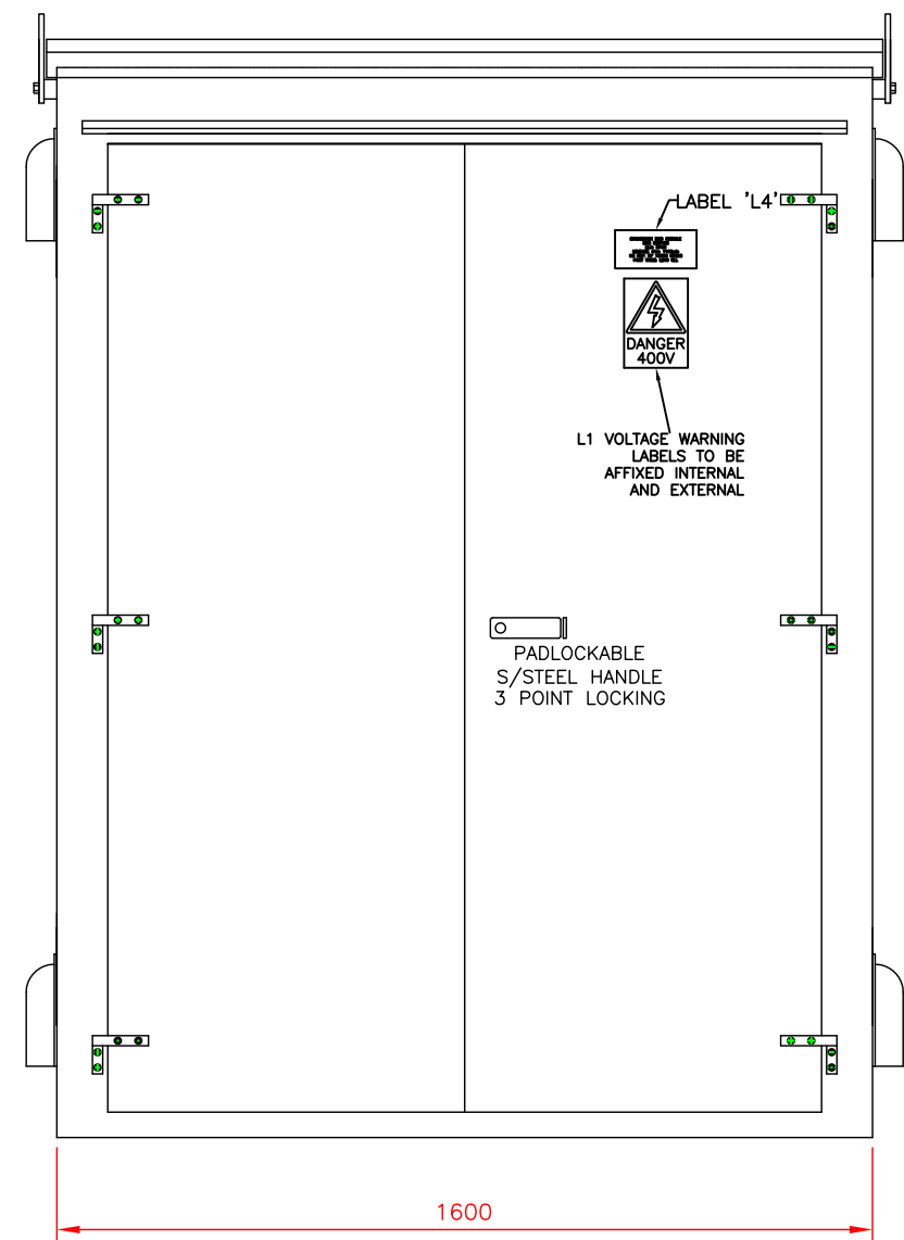
REAR ELEVATION
