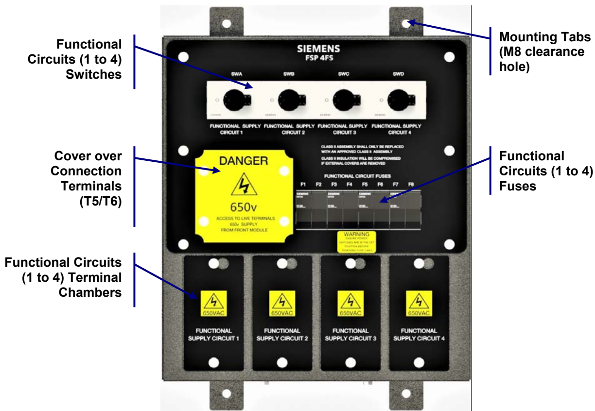
Figure 3: FSP Rear Module (4 Output) Layout Arrangement
