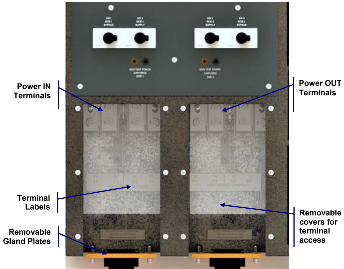
Figure 5: Power In/Out Terminal Arrangement
