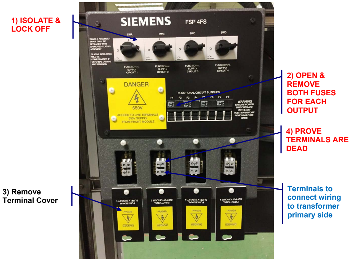
Figure 17: Termination of Hybrid Transformer Primary Feed Cables
