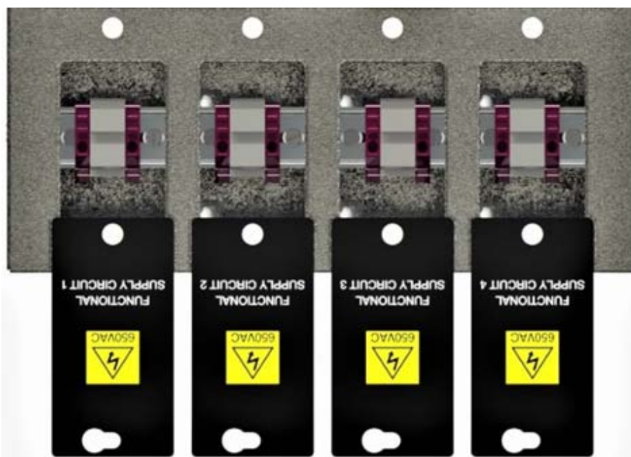
Figure 4: FSP Rear Module (4 Output) Functional Supply Terminals
