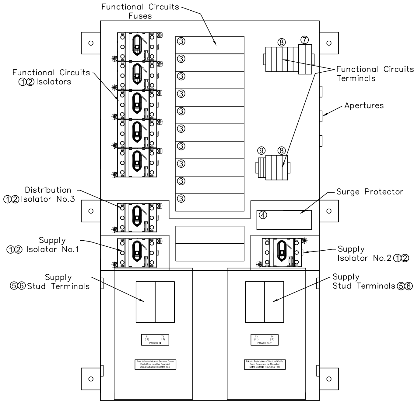
VIEW WITH COVERS REMOVED
